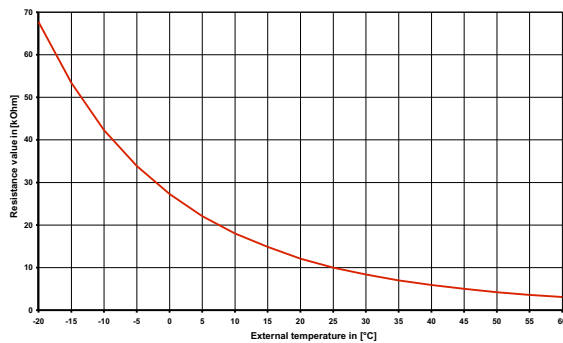
Fig. 7.1: Sensor characteristic curve NTC-10
