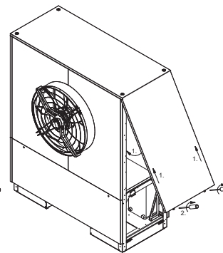
Closing the lateral and rear cover panels on top
