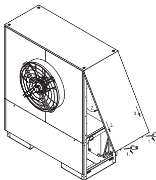
Opening the lateral and rear cover panels on top
