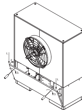
Closing the lower covers
